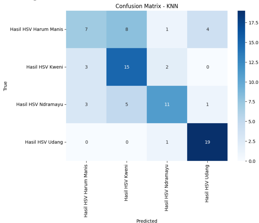
Gambar 4. Confusion Matrix metode KNN
